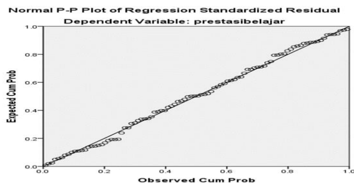
Gambar 1. Kurva Normal Probability P-Plot
