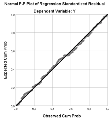
Gambar 1. Normal P-Plot
