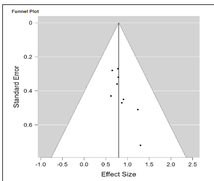
Gambar 1. Funnel Plot
