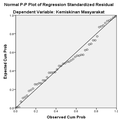
Gambar 2. Grafik Probability Plot
