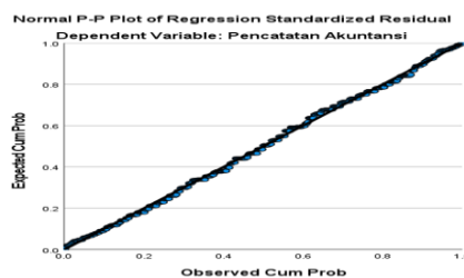
Gambar 1. Hasil Uji Normalitas Grafik Probability Plot (P-Plot)
