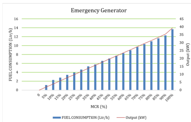
Correlation of Fuel Consumption of Emergency Generator with Electrical Power Output (analysis)
