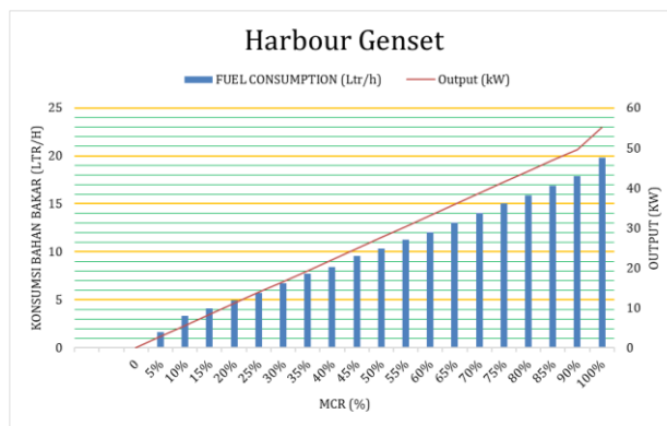
Correlation of Fuel Consumption of Harbour Generator with Electrical Power Output (analysis)
