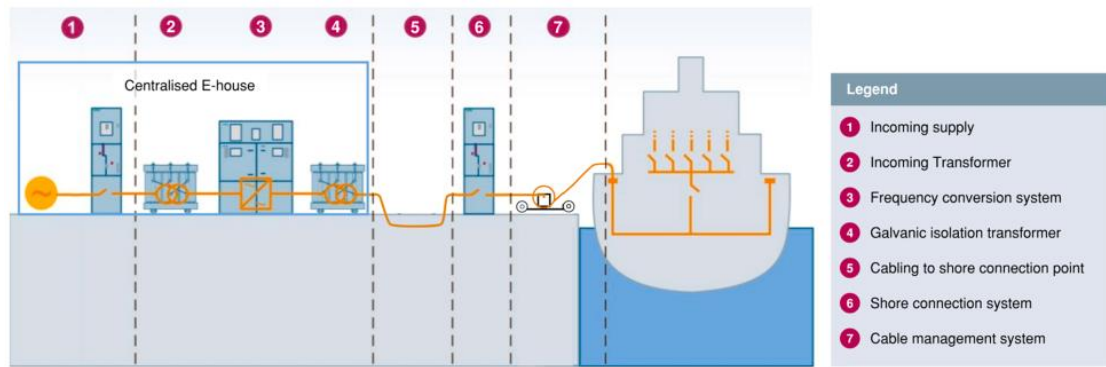
Shore Side Electricity system (Bullock et al., 2023)
