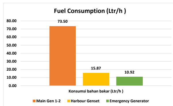
Fuel Consumption Comparison (analysis, 2024)
