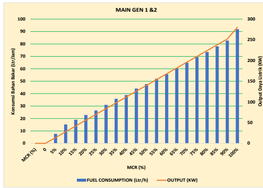
Correlation of Fuel Consumption of Auxiliary Motors 1 and 2 with Electrical Power Output (analysis)
