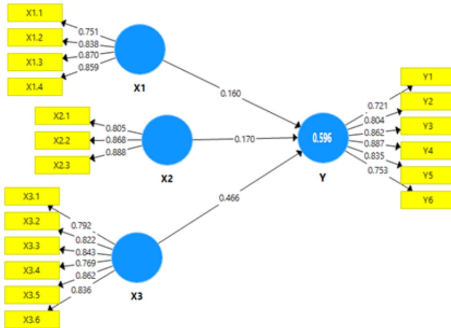
Gambar 3 Output PLS Algorithm
